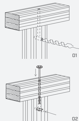
SIMPLEX ASSEMBLY
